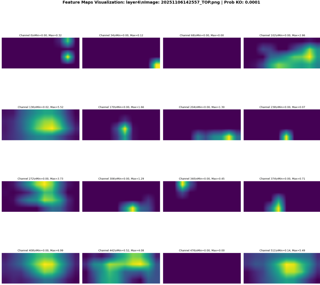
Figure 7: Intermediate feature map activations from layer4 . The network encodes complex spatial relationships and textures within the PCL region.
